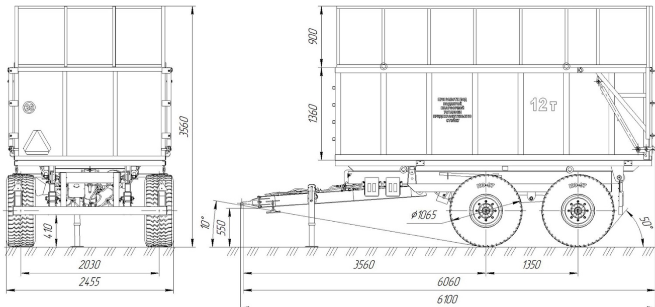
Image 1.4 – Semi-trailer version PTS-12CH
