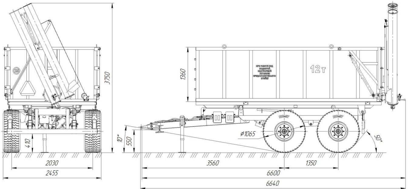
Image 1.3 – Semi-trailer version PTS-12P
